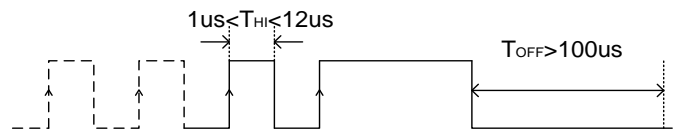
Figure 15. sequence diagram of line pulse
