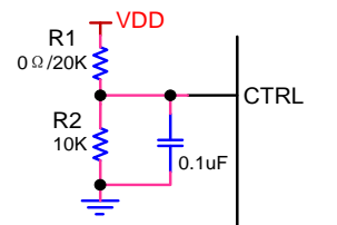
Figure 15. The LPA2176 sets the working mode with hardware
